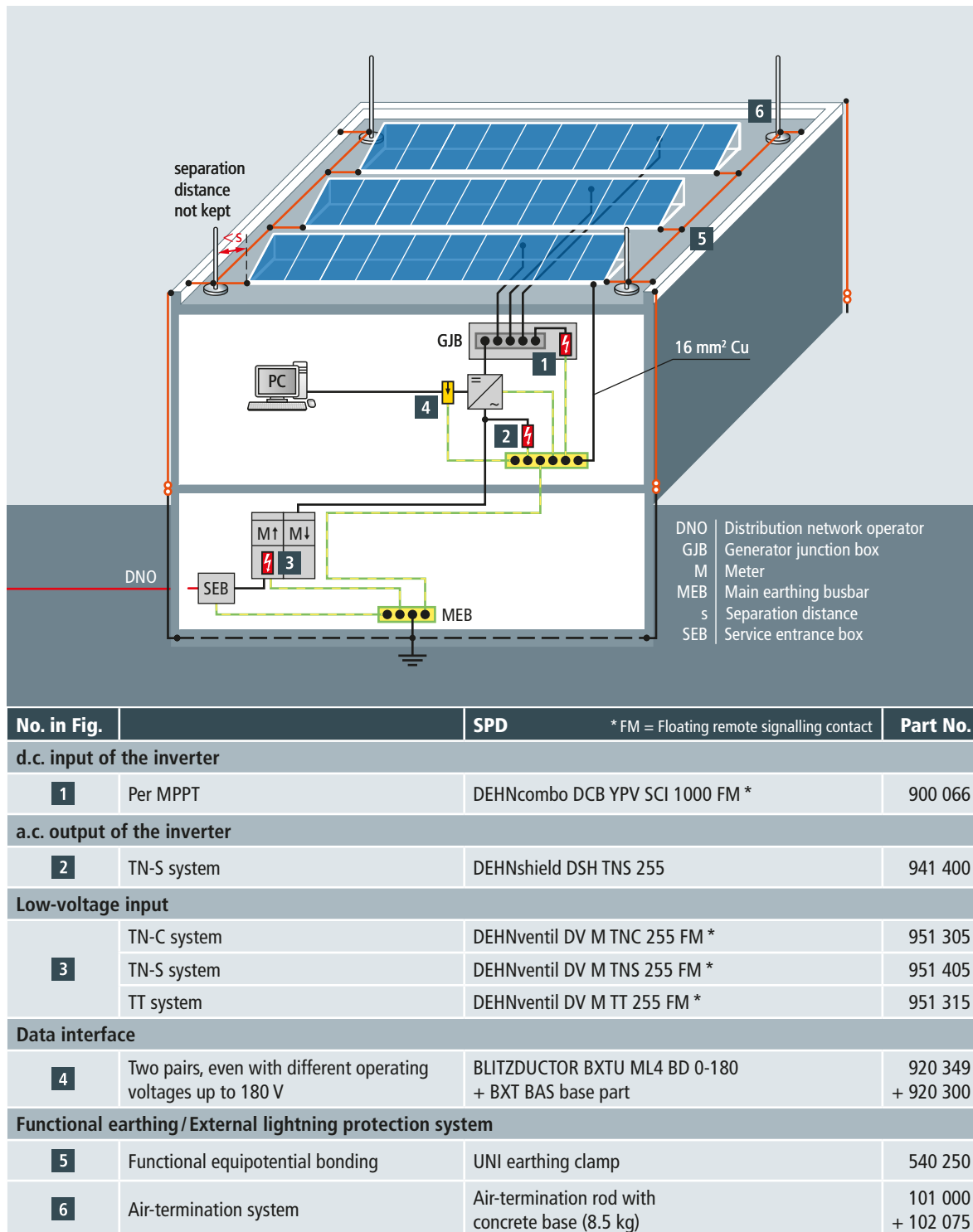
Figure 17 Building with external LPS and insufficient separation distance – situation C (Supplement 5 of the DIN EN 62305-3 standard)
