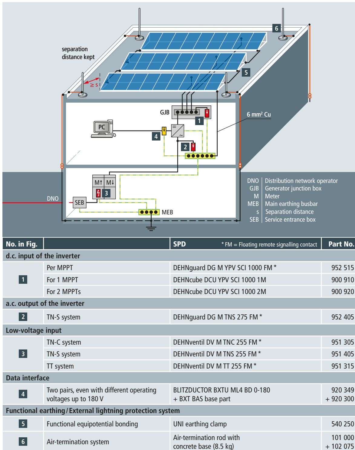
Figure 13 Building with external LPS and sufficient separation distance – situation B (Supplement 5 of the DIN EN 62305-3 standard)
