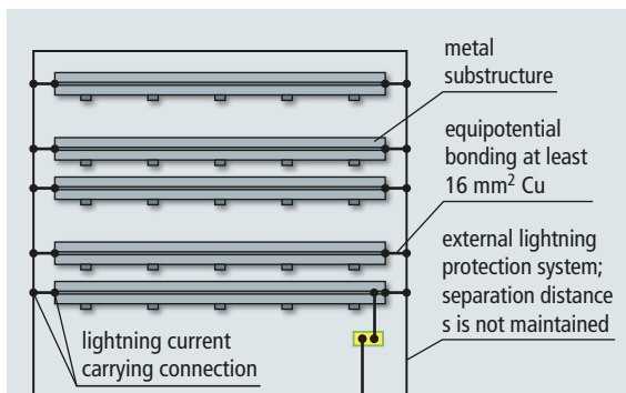
Figure 2 Lightning equipotential bonding for the mounting systems if the separation distance is not maintained
