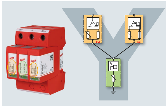
Figure 9 Modular DEHNgard M YPV SCI ... (FM) type 2 surge arrester with fault-resistant Y circuit and three-step d.c. switching device
