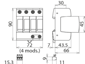
Dimension drawing DG M TT CI 275 FM
