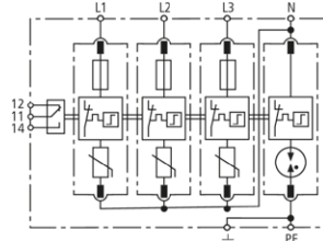
Basic circuit diagram DG M TT CI 275 FM
