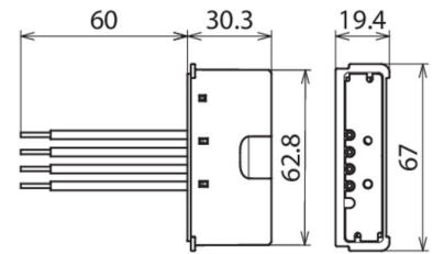
Dimension drawing DCOR L 2P SN1864
