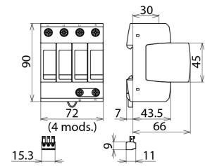
Dimension drawing DG M TT 320 FM
