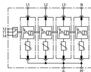
Basic circuit diagram DG M TNS 385 FM
